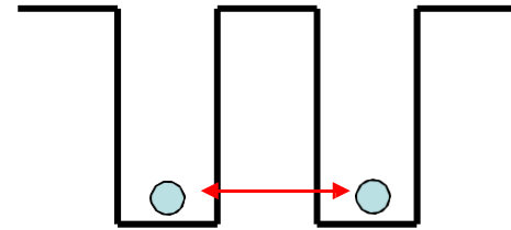
tunneling
