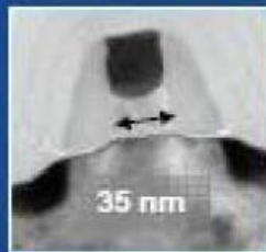
SiGe S/D Strained Silicon
