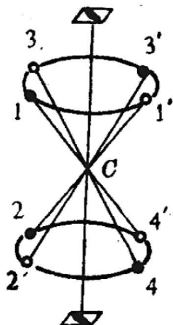
(e) \bar{4}
