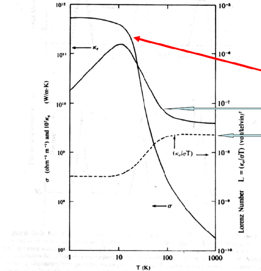
Figure 3-1 Temperature dependence of the electrical conductivity \sigma and the electronic thermal conductivity \kappa_e for highly pure copper.
